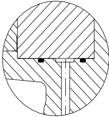
Seal Sleeve O-Ring
