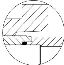
Seal Sleeve O-Ring
